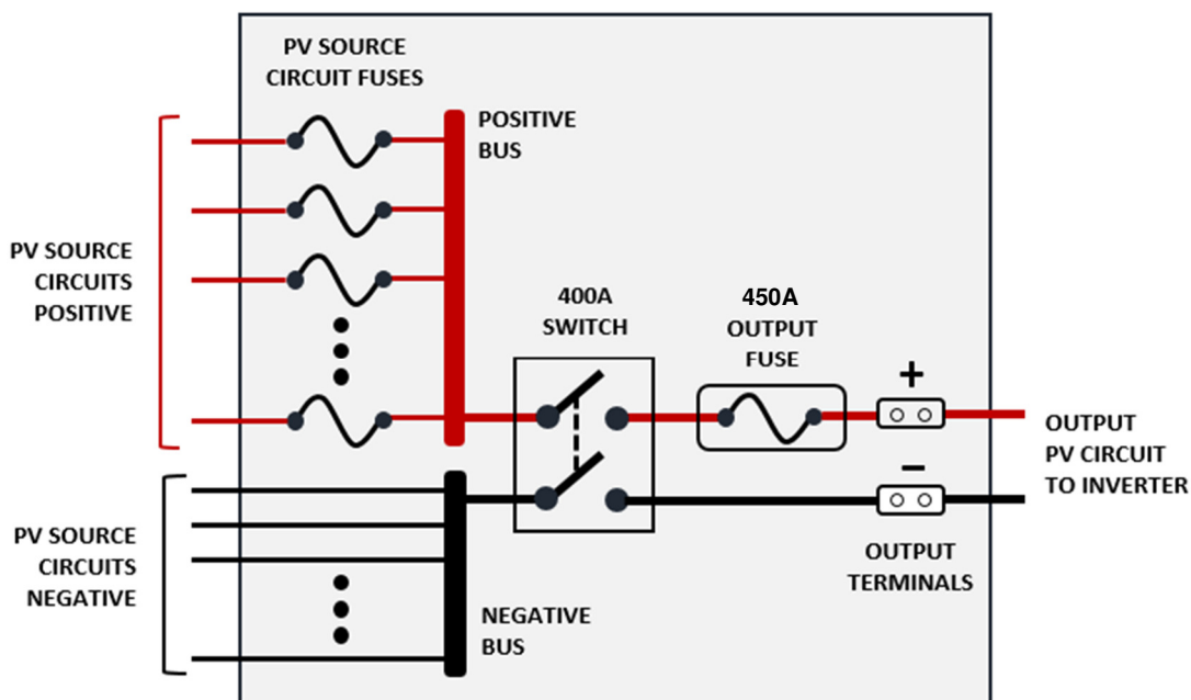
Figure 2.4 – Schematic of the CR1500-xxP-yyF-400S Combiner (Note: the CR1500-xxP-yyF-250S Combiner is similar, but with a 250A switch and 315A output fuse.)
