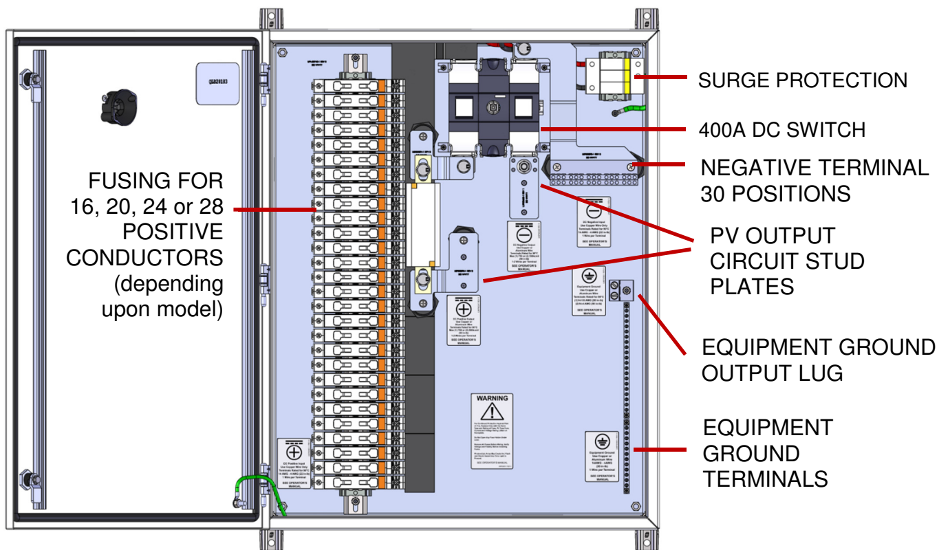
Figure 2.3 - The CR1500-xxP-yyF-400S Combiner
