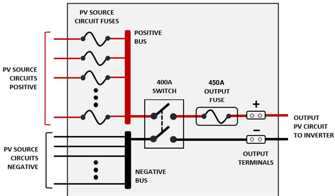
Figure 2.4 – Schematic of the CR150-xxP-yyF-400S Combiner (Note: the CR150-xxP-yyF-250S Combiner is similar, but with a 250A switch and 315A output fuse.)
