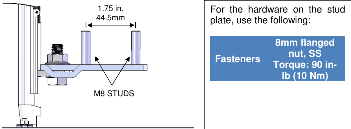
Figure 4.5 – Stud Plate Elevation View
